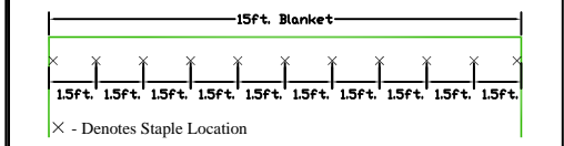
Figure D - Plan View
